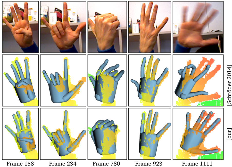
Figure 6.20: A few comparison frames illustrating the difference in performance of our method compared to (Schröder et al. 2014). From left to right we can observe problems related to: correspondences to the back of the model, lack of silhouette energy (3 times) and loss of tracking due to fast motion.
