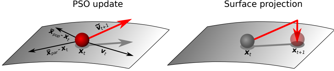
Figure 3.10: Illustration of a PSO update for one marker position. First, the new velocity \tilde{\mathbf{v}}_{t+1} of the marker is computed as a weighted linear combination of the vectors towards the particle's local optimum \bar{\mathbf{x}}_{\text{par}} - \mathbf{x}_t , the population's global optimum \bar{\mathbf{x}}_{\text{pop}} - \mathbf{x}_t and the particle's current velocity vector \mathbf{v}_t . This update can send the marker off the surface of the hand model due to the curvature of the model surface. Therefore, in a second step, the new position \mathbf{x}_{t+1} is computed by projecting back onto the surface. The velocity \mathbf{v}_{t+1} is then recomputed accordingly.
