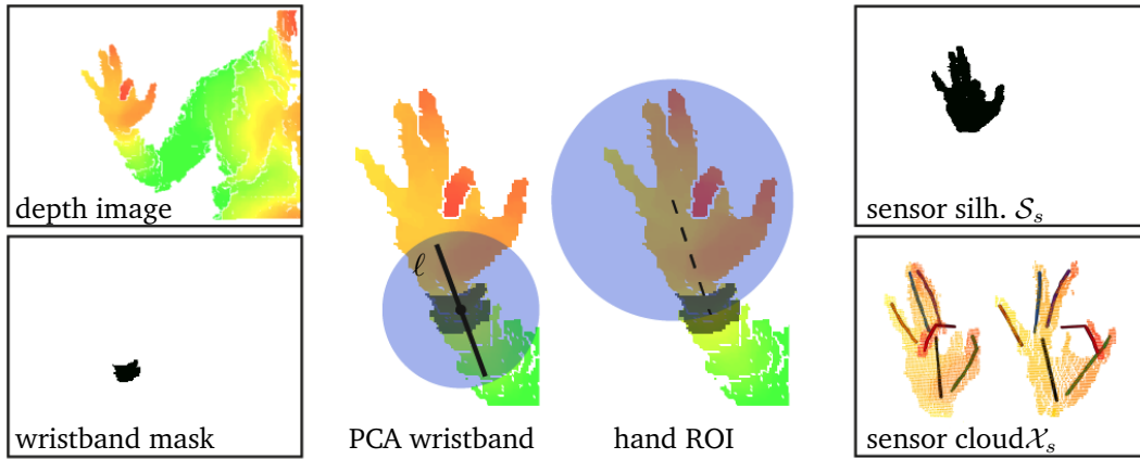
Figure 6.5: We first identify the wristband mask by color segmentation, then compute the 3D orientation of the forearm as the PCA axis of points in its proximity. Offsetting a 3D sphere from the wristband center allows isolating the region of interest. The obtained silhouette image and sensor point clouds are shown on the right.
