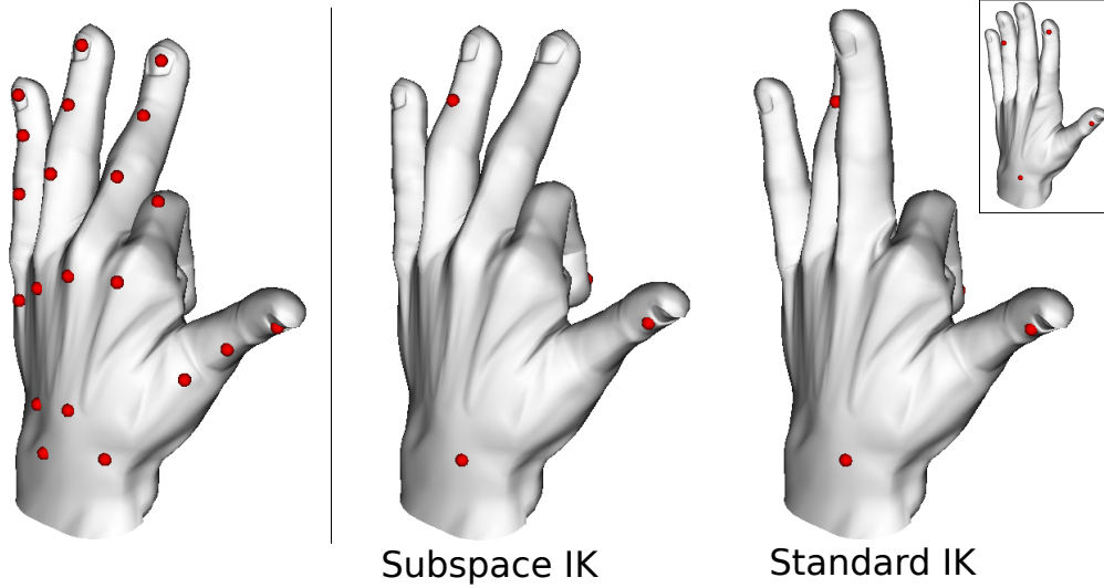
Figure 3.6: Full and reduced marker sets and reconstructed hand postures with standard inverse kinematics optimizing for all joint angles and subspace inverse kinematics optimizing for reduced subspace parameters. While the standard approach cannot articulate the markerless fingers, the subspace approach captures the correlations between fingers and articulates them using the reduced marker set.
