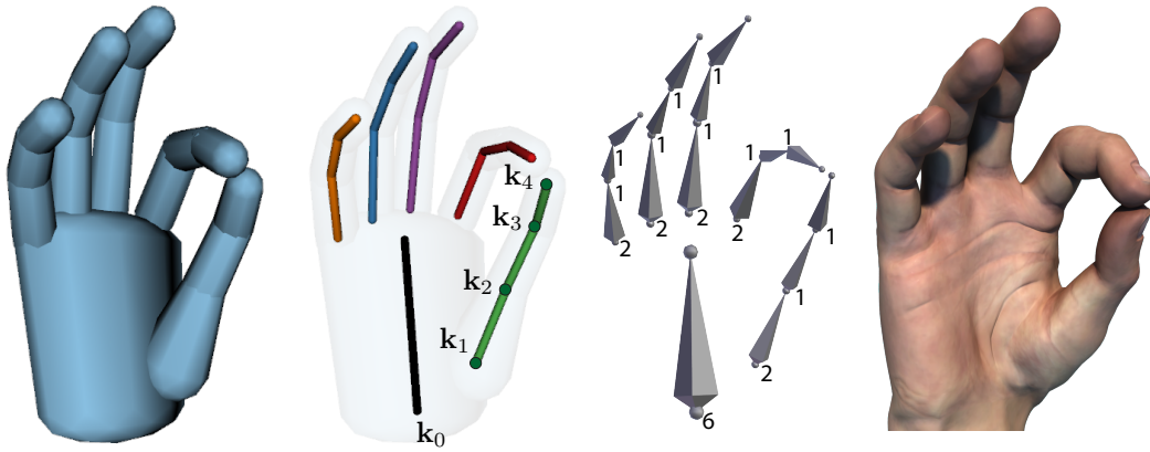
Figure 6.4: A visualization of the template hand model with the number and location of degrees of freedom of our optimization. From left to right: The cylinder model used for tracking, the skeleton, the BVH skeleton exported to Maya to drive the rendering, the rendered hand model.
