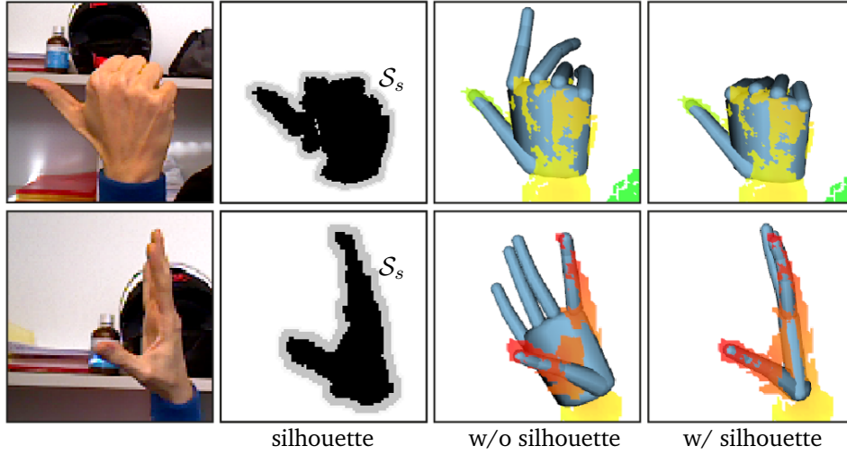
Figure 6.9: Our 2D silhouette registration energy is essential to avoid tracking errors for occluded parts of the hand. When no depth data is available for certain parts of the model, a plausible posture is inferred by ensuring that the model is contained within the sensor silhouette image \mathcal{S}_s .
