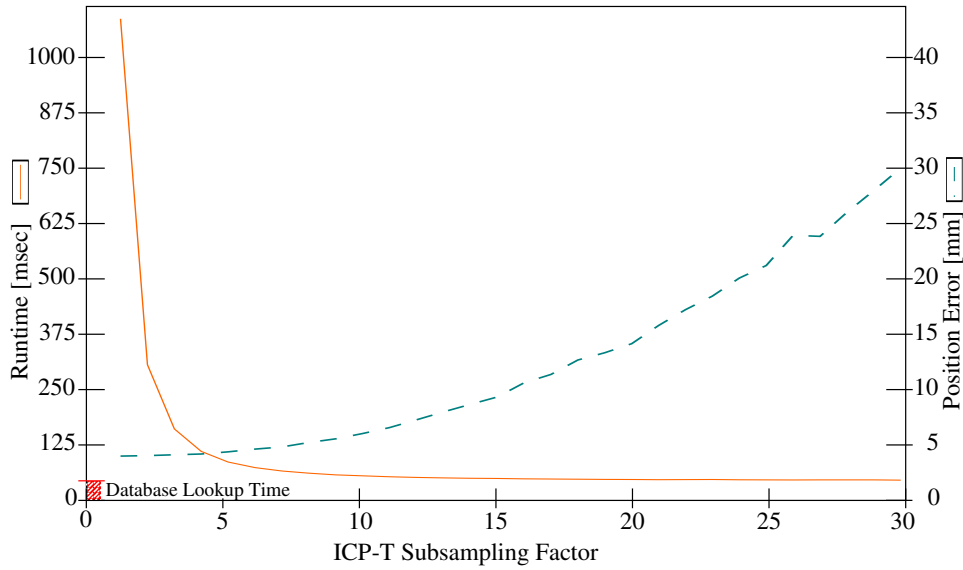
Figure 4.11: Overall runtime and position estimation error in regard to an increasing point cloud subsampling factor.
