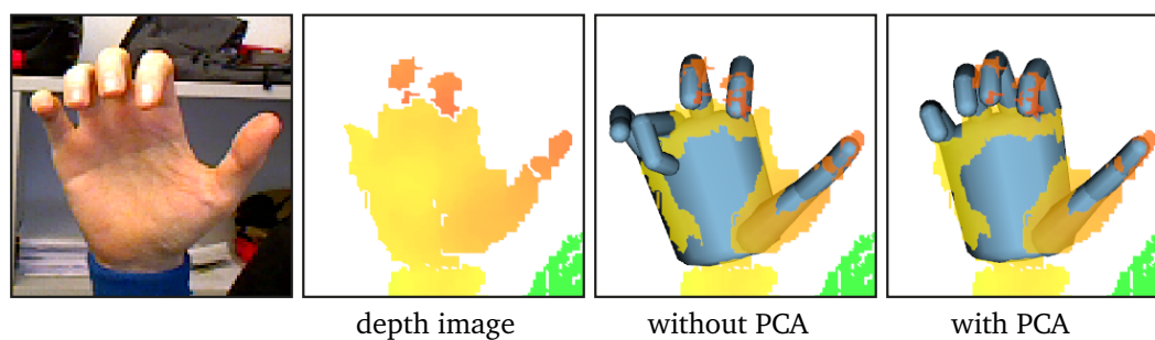
Figure 6.13: Our posture-space regularization using a PCA prior ensures that a meaningful posture is recovered even when significant holes occur in the input data.
